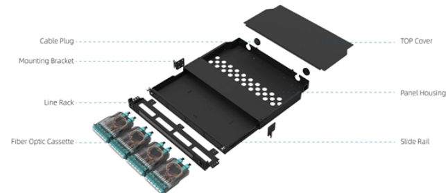
Component Diagram
